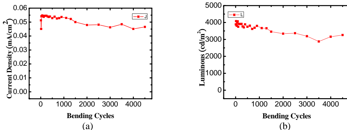
Fig. 2 (a) Current efficiency and (b) luminance under different bending cycles.
