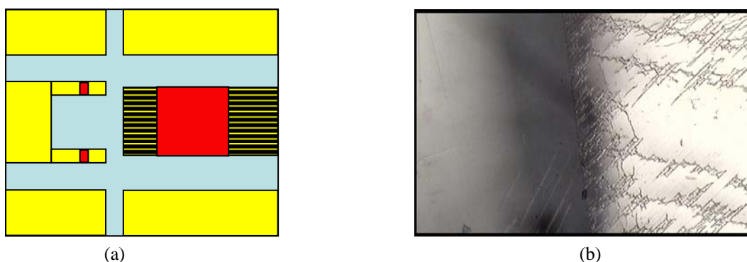
Fig. 3 (a) Structure of Flexible OLED surface. (b) Interface of ITO and Substrate.
